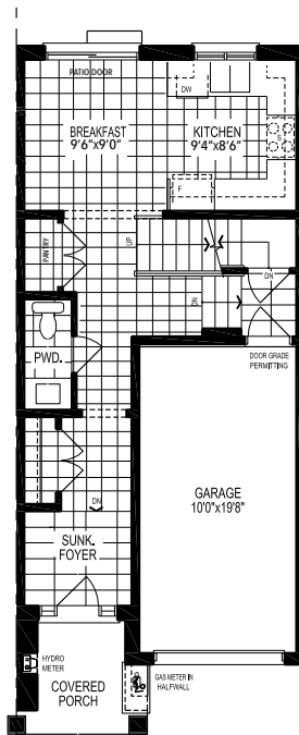
GROUND FLOOR PLAN, EL. '1802-A' & '1802-A-MOD'
