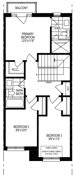
THIRD FLOOR PLAN, EL. '1802-A' & '1802-A-MOD'
