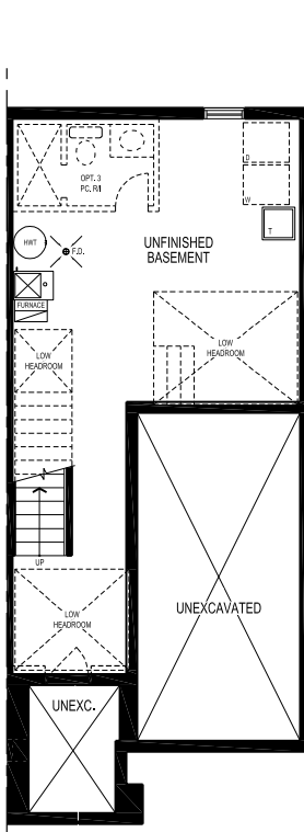
BASEMENT PLAN, EL. '1801-A'
