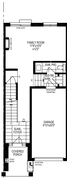
GROUND FLOOR PLAN, EL. '1801-A'
