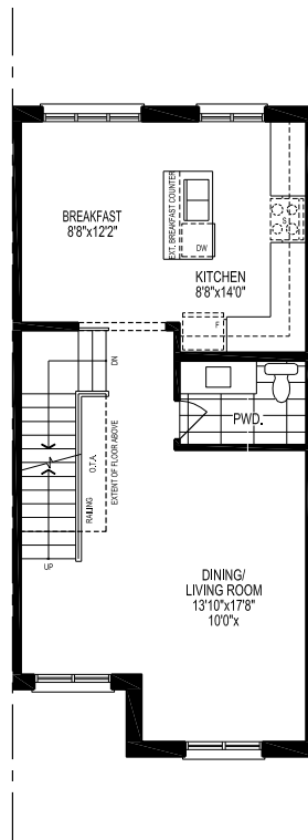
MAIN FLOOR PLAN, EL. '1801-A'
