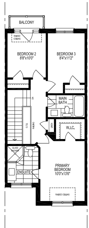
THIRD FLOOR PLAN, EL. '1801-A'
