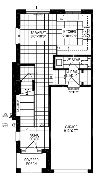
GROUND FLOOR PLAN, EL. '1803-A'
