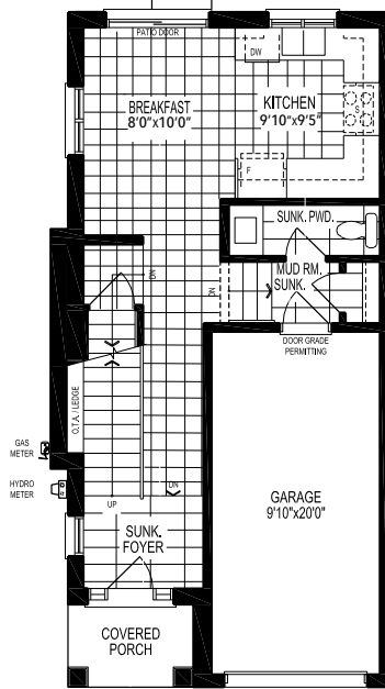
GROUND FLOOR PLAN, EL. '1803-A'
