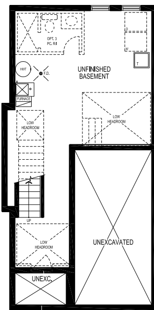
BASEMENT PLAN, EL. '1803-A'
