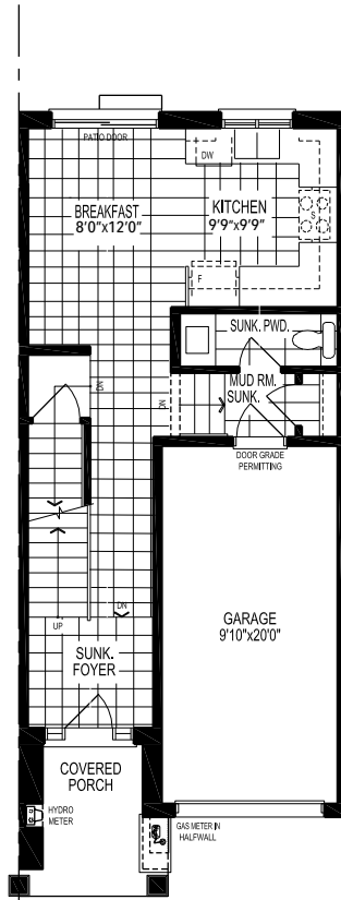
GROUND FLOOR PLAN, EL. '1801-A'
