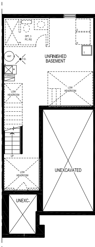
BASEMENT PLAN, EL. '1801-A'
